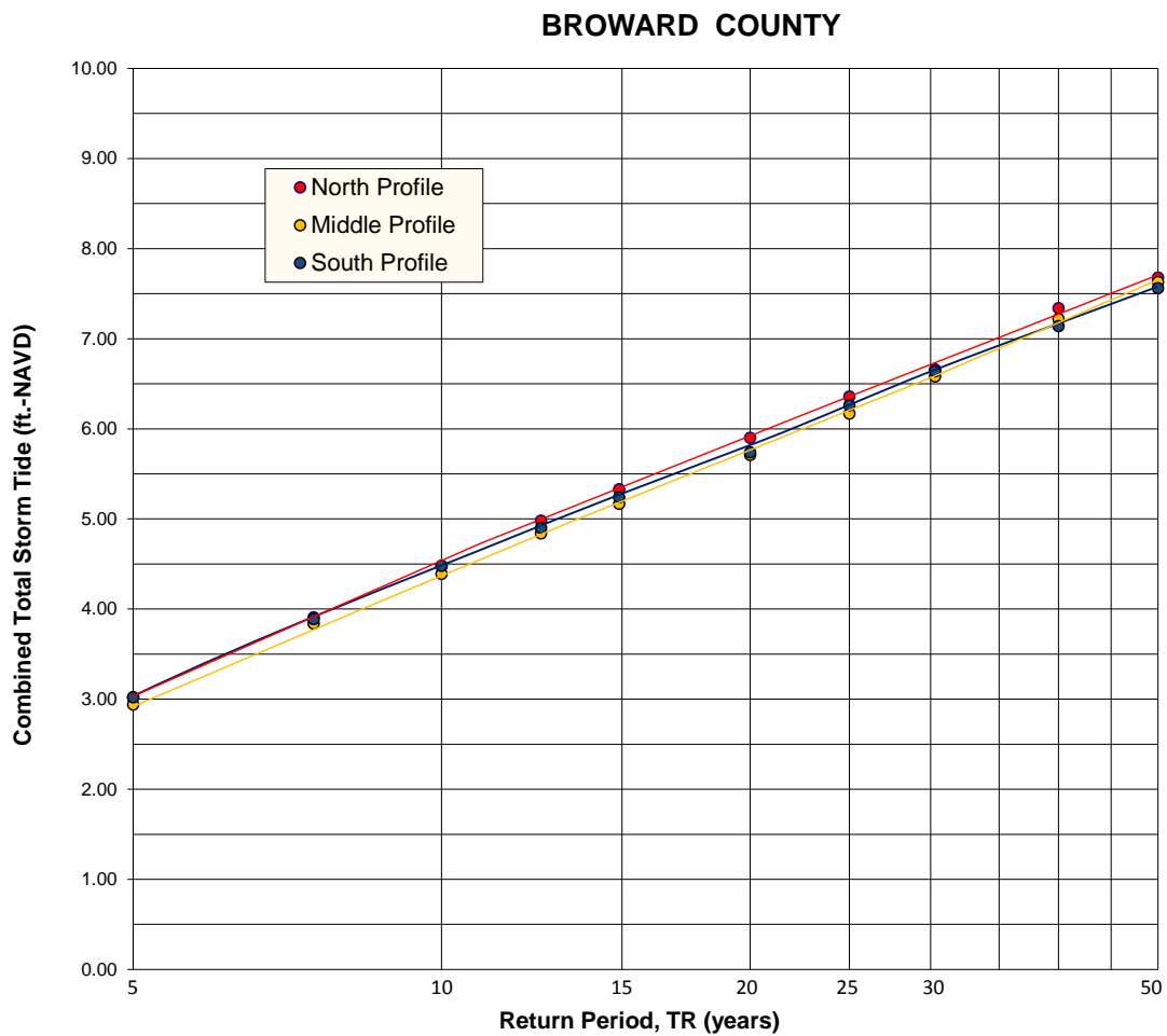
Figure 10: Combined Total Storm Tide Elevation versus Return Period for Study Area
