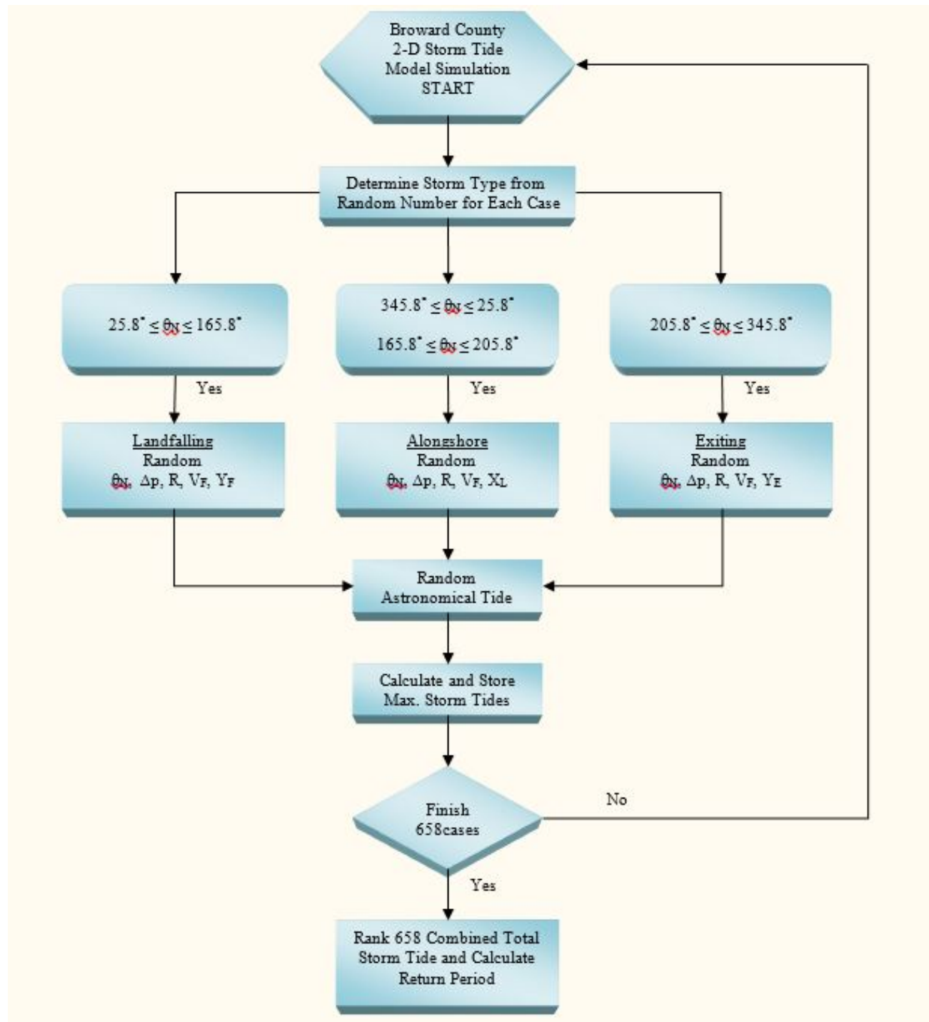
Figure 9: Flow Chart for Two-Dimensional Storm Tide Simulations
